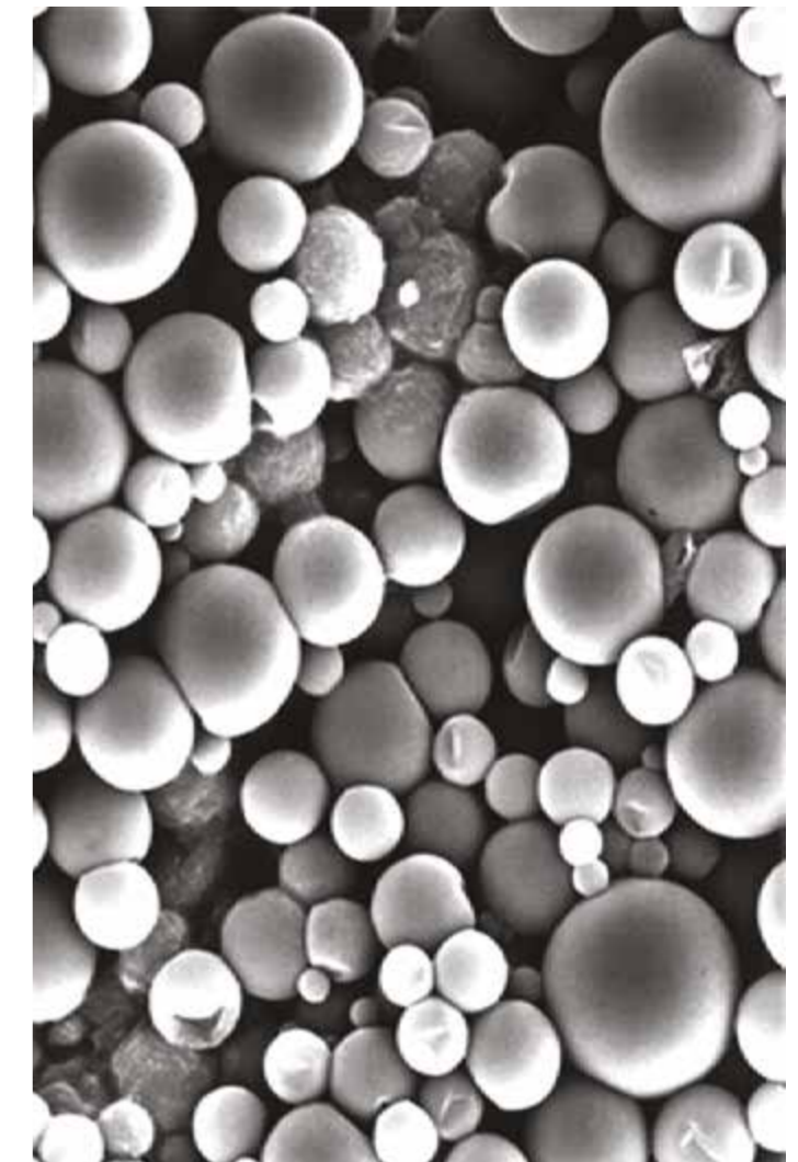
Figure 4: Electron Micrograph of the Trojan® microcapsule
